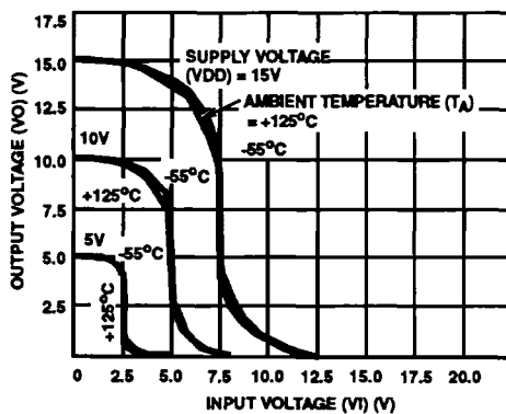
FIGURE 3. TYPICAL VOLTAGE TRANSFER CHARACTERISTICS AS A FUNCTION OF TEMPERATURE
