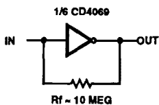
FIGURE 15. HIGH-INPUT IMPEDANCE AMPLIFIER
