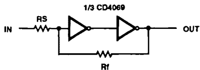
UPPER SWITCHING POINT
