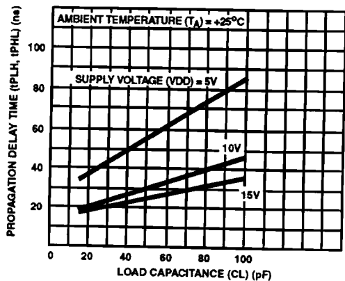
FIGURE 9. TYPICAL PROPAGATION DELAY TIME vs LOAD CAPACITANCE
