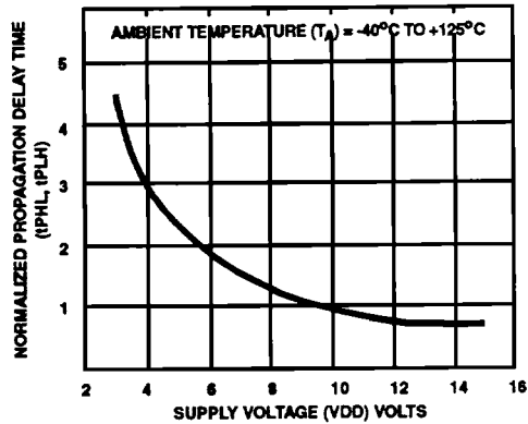
FIGURE 13. VARIATION OF NORMALIZED PROPAGATION DELAY TIME (tPHL AND tPLH) WITH SUPPLY VOLTAGE
