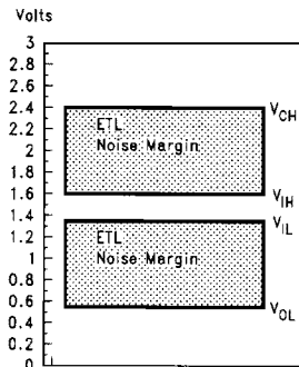
ETL Worst Case V_{OUT}-V_{IN}
