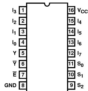
CD74FCT151, CD74FCT2151T (QSOP, SOIC) TOP VIEW
