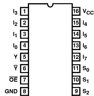
CD74FCT251 (QSOP, SOIC) TOP VIEW
