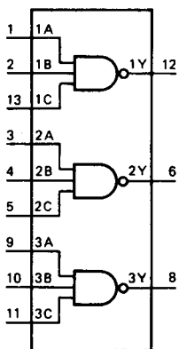
Fig. 1 Logic symbol
