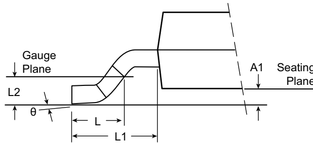
View B
