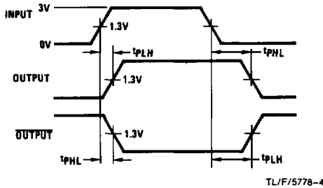
FIGURE 2. Propagation Delays
