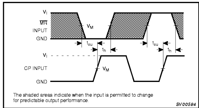
Figure 4. \overline{MR} set-up and hold times.
