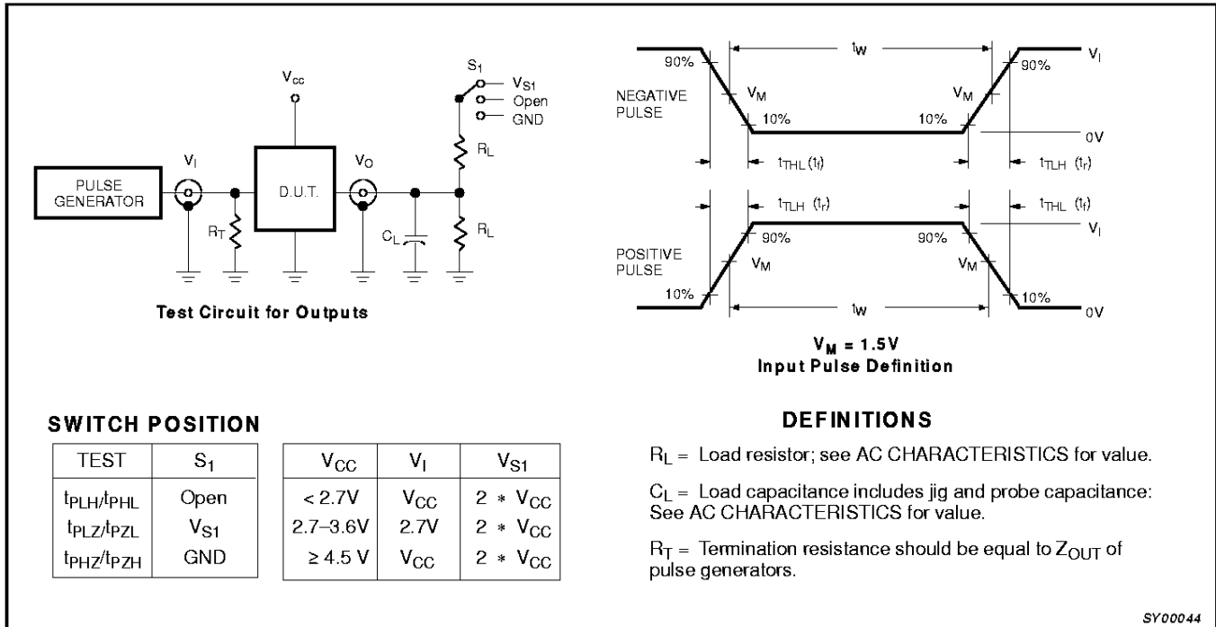
Figure 6. Load circuitry for switching times.
