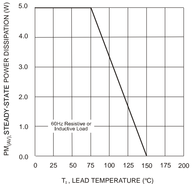
Figure 6. Steady-State Power Derating Curve
