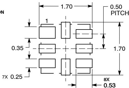
DIMENSIONS: MILLIMETERS
