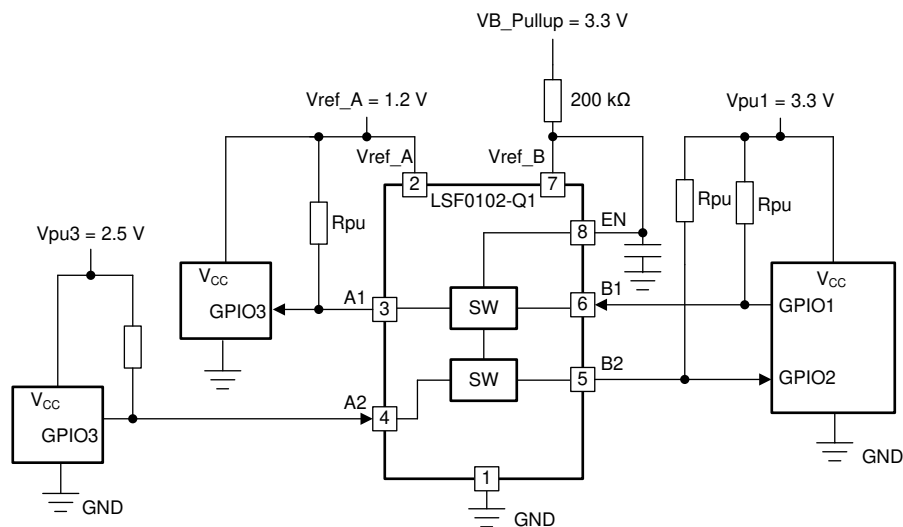
图 8-1. Bidirectional Translation to Multiple Voltage Levels
