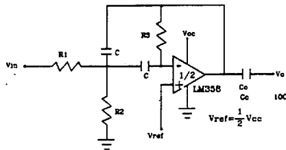
FIGURE 2 - MULTIPLE FEEDBACK BANDPASSFILTER
