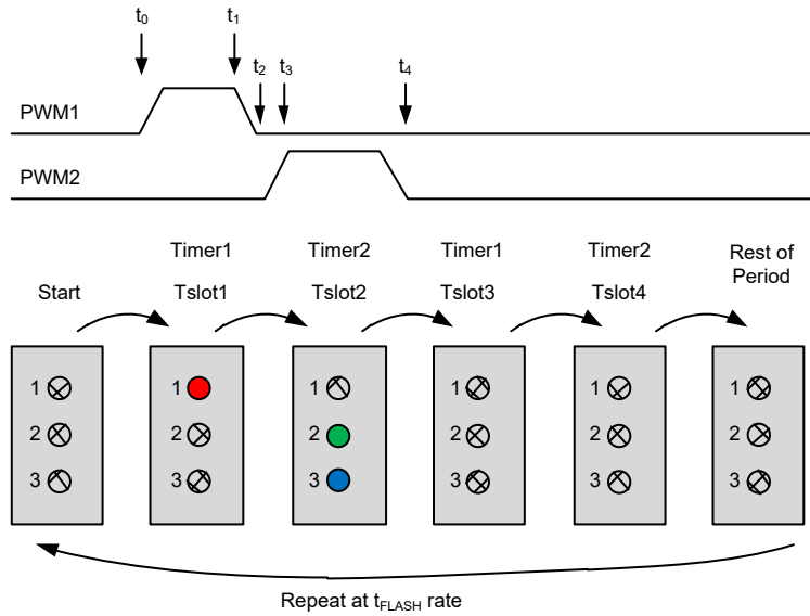
Figure 6. Timer Slot2 Example
