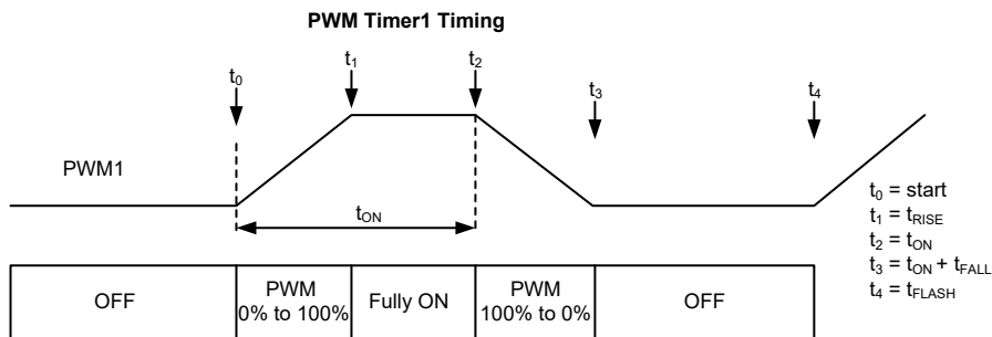
Figure 4. Channel Timing Diagram
