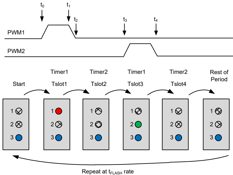
Figure 7. Timer Slot3 Example
