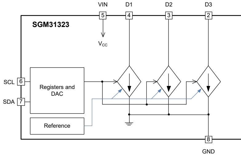
Figure 3. Block Diagram
