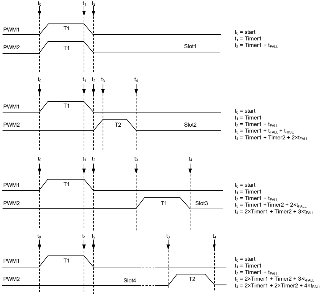
Figure 5. Timer Slot Timing Diagram
