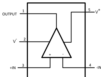
DBV and DCK Package 5-Pin SOT-23 and SC70 Top View
