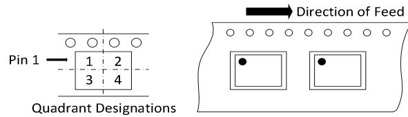
Figure 12.3 Reel Information of SOP8(150mil)
