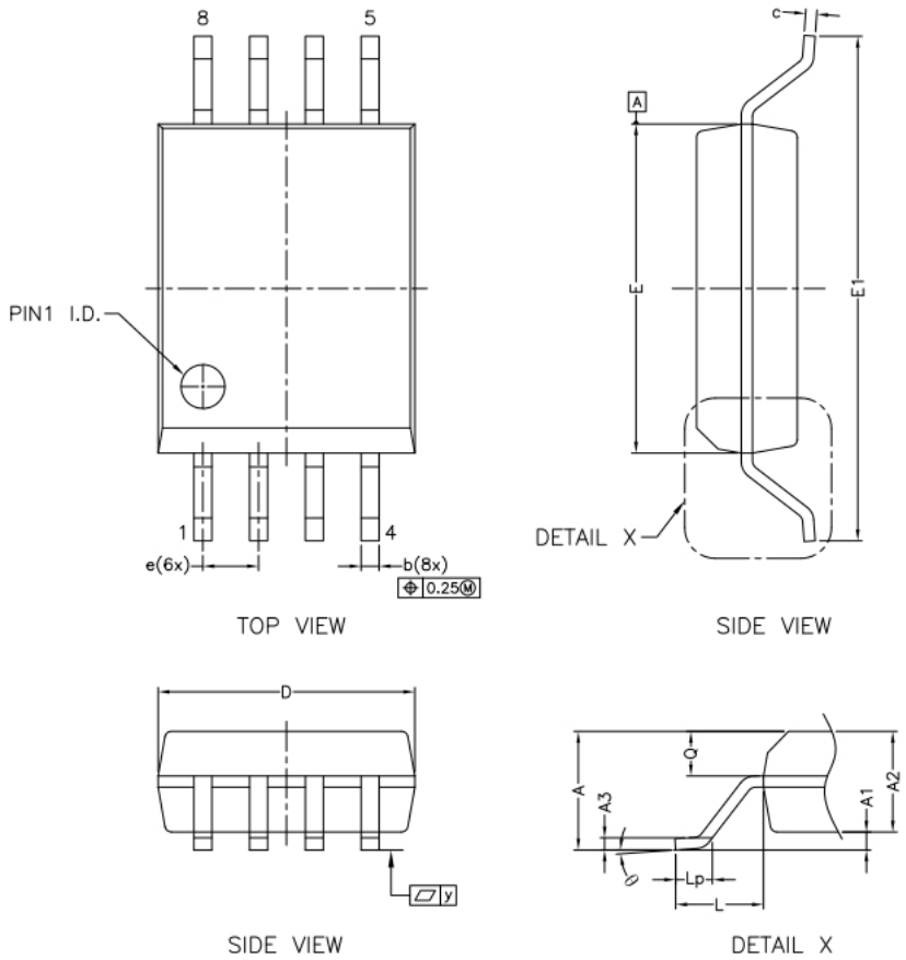
Figure 9.1 SOW8 Package Shape and Dimension in millimeters
