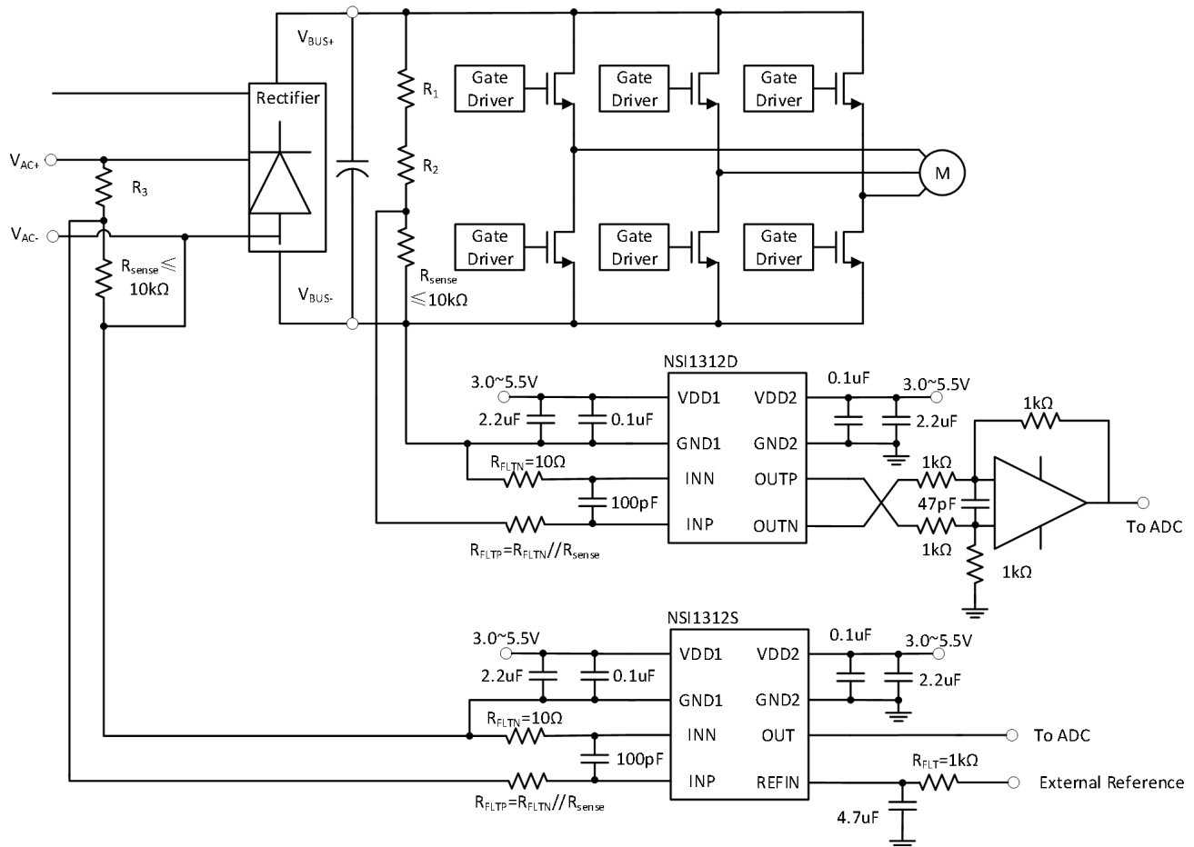
Figure 8.1 Typical application circuit in voltage sensing
