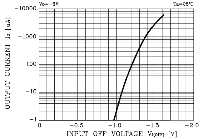
Fig. 2 I_o - V_{I(OFF)}
