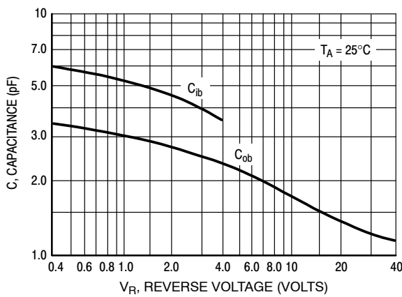
Figure 7. Capacitances
