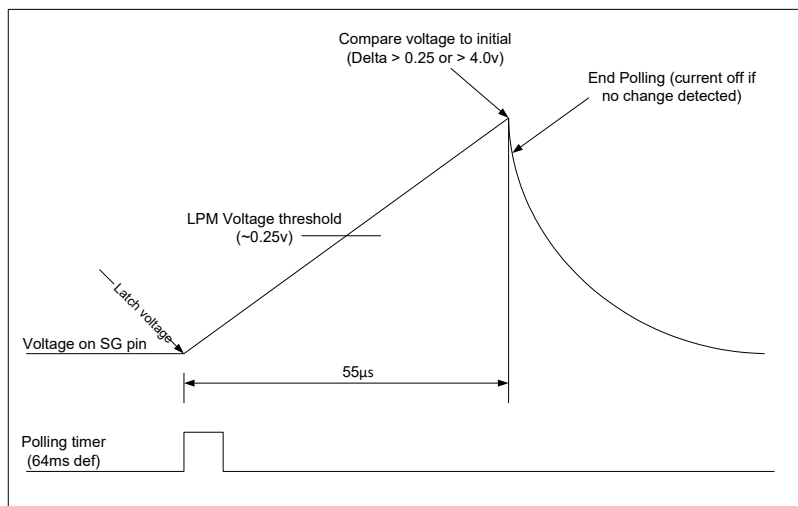
Figure 12. Low-power mode polling check
