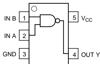
Figure 1. Pinout
