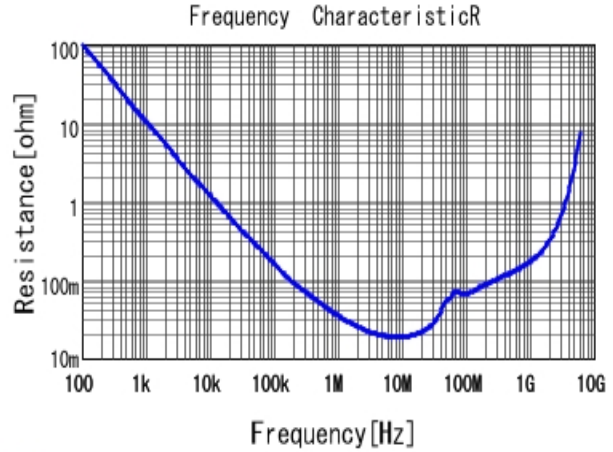
■ GRM188R61E104KA01 R DCOV, 25degC
