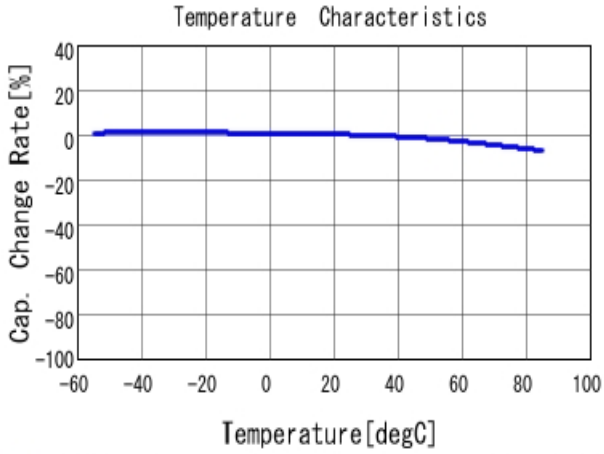
■ GRM188R61E104KA01 C-Temp. capchange, DC0.0V, AC1.0V r m
