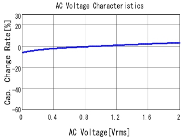
■ GRM188R61E104KA01 C-AC Voltage capchange, DCOV, 25.0d
