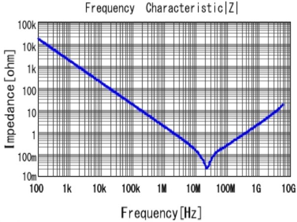
■ GRM188R61E104KA01 |Z| DCOV, 25degC
