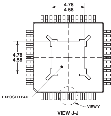
VIEW J-J
